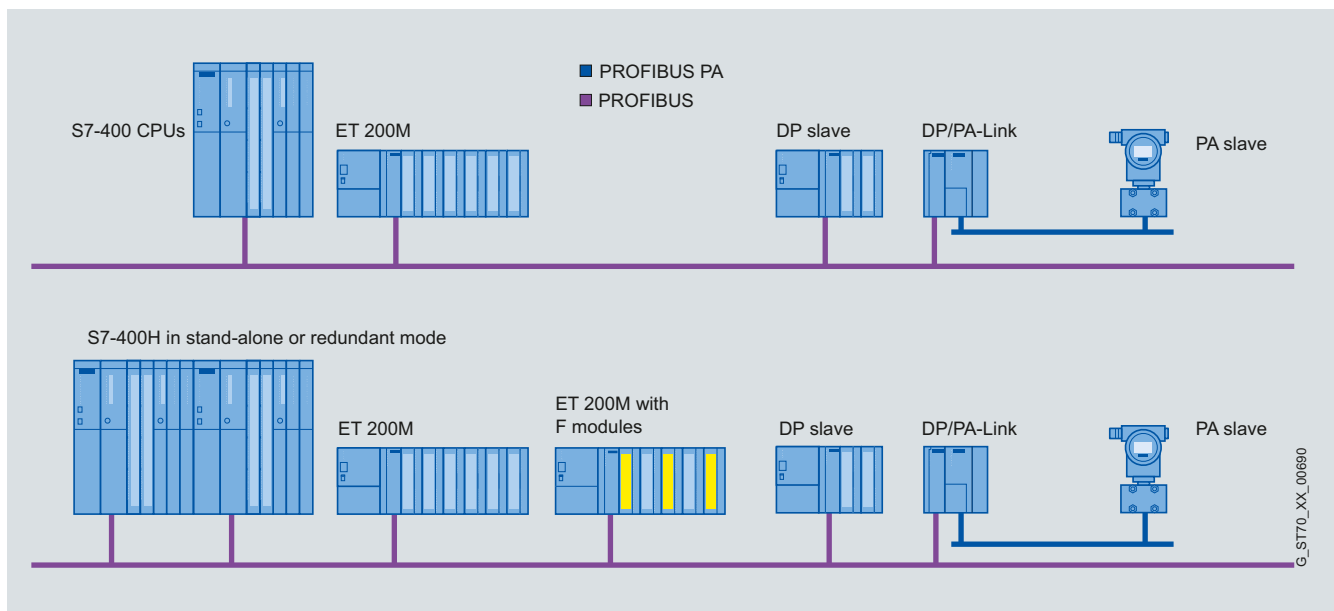
Range of modules that can be added to or removed from a plant during operation with an S7-400 as master
