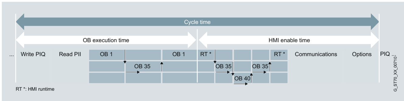
Cycle diagram for SIMATIC WinAC MP with control and HMI segments
