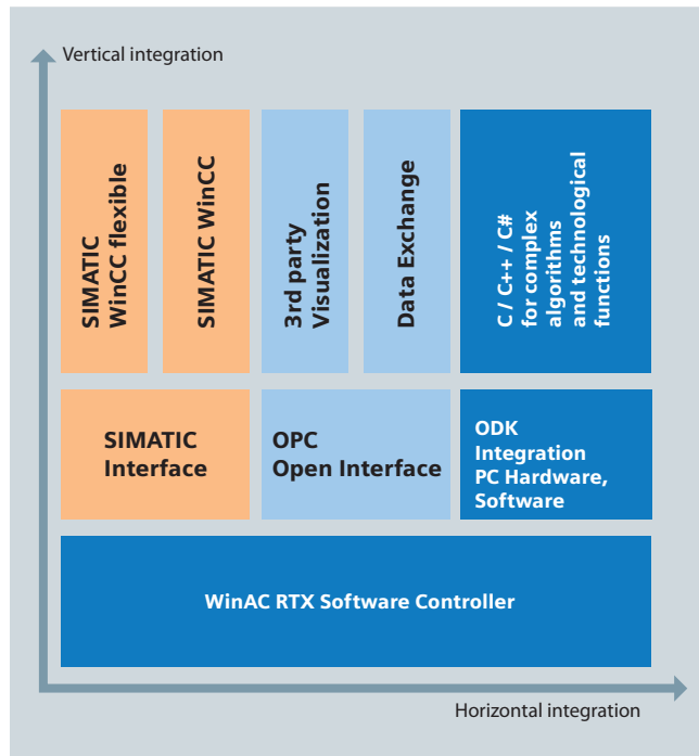
WinAC RTX offers open data interfaces for vertical and horizontal integration of other applications
