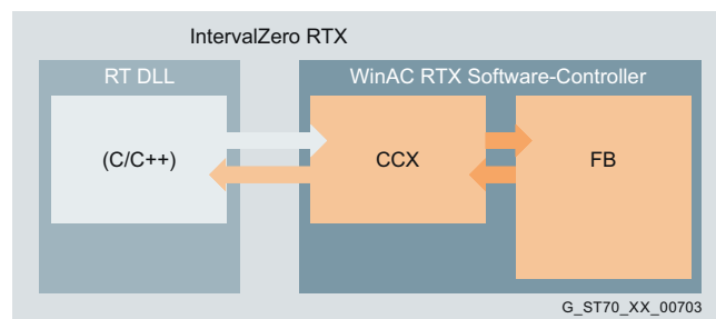
The Custom Code Extension Interface (CCX) offers the facility of calling high-level language programs from the control program of the WinAC software controller
